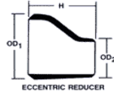
ECCENTRIC REDUCER
