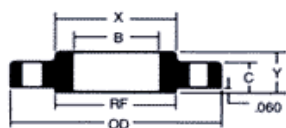
SLIP-ON
